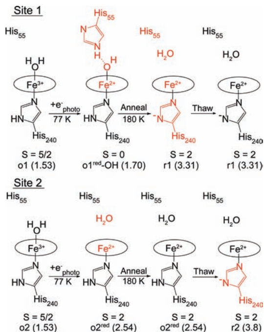
Figure 13. Heme states observed from the cryoreduction of oxidized TDO with spin states as shown. The numbers in parentheses are the values of \Delta E_Q (in mm/s) for the respective states. Red indicates a change from the previous state.
