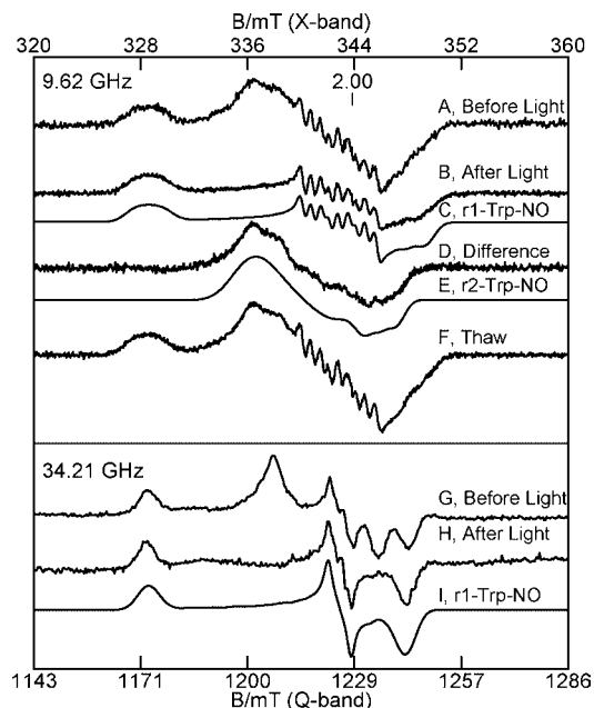
Figure 9. Photodissociation of the NO adduct from r2-Trp-NO. X- (top part) and Q-band (lower part) EPR spectra of the NO adduct of 0.3 mM reduced TDO with 10 equiv of L-Trp. (A) Before light, (B) after exposure to light at 77 K, (C) simulation of r1-Trp-NO, (D) difference (A)–(B), (E) simulation of r2-Trp-NO, (F) after anaerobic thawing in dark, (G) before light, (H) after exposure to light at 77 K, and (I) simulation of r1-Trp-NO. The experimental conditions and simulation parameters of the species are the same as in Figure 8.
