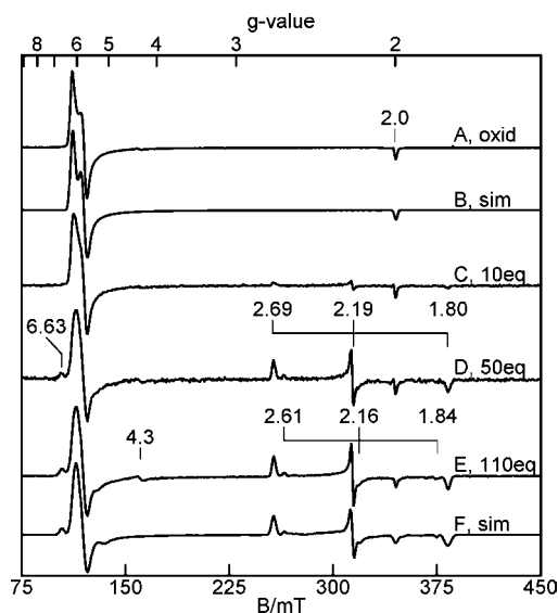
Figure 1. EPR spectra of 220 \mu\text{M} oxidized TDO, pH 7.4. (A) As-isolated, (B) simulation of (A), (C) with 10 equiv of L-Trp, (D) with 50 equiv of L-Trp, (E) with 110 equiv of L-Trp, and (F) simulation of (E). Experimental conditions: microwaves, 0.2 mW at 9.65 GHz; temperature, 11 K. See text and Table 1 for simulation parameters.
