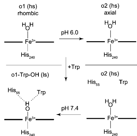
Figure 12. Spectroscopic states observed for oxidized TDO.
