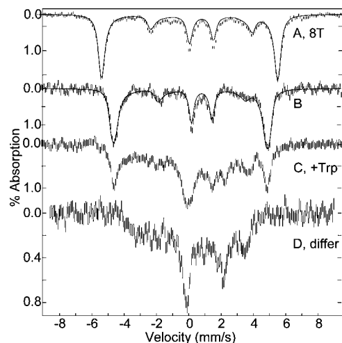
Figure 3. Mössbauer spectra of 1 mM oxidized TDO, pH 7.4. (A) Oxidized TDO in a magnetic field of 8 T, (B) oxidized TDO, (C) with L-Trp, (D) difference spectrum of (C) – 0.4 (B). Experimental conditions: temperature, 4.2 K; magnetic field of 45 mT (except (A)) parallel to \gamma -ray direction. The solid lines are least-squares fits with parameters given in the text.
