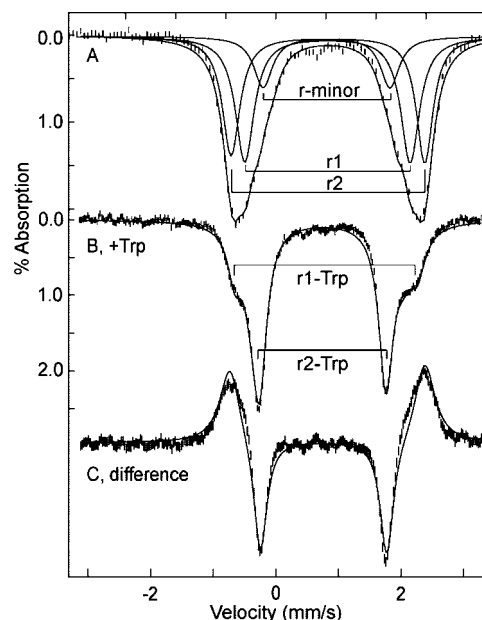
Figure 4. Mössbauer spectrum of 1 mM TDO, pH 7.4. (A) Reduced, (B) reduced with 10 equiv of L-Trp, (C) difference spectrum (B) – (A) for equal areas of (A) and (B). All spectra recorded at 4.2 K in a magnetic field of 45 mT parallel to \gamma -ray direction. The solid lines overlaid on the data are least-squares fits using the parameters given in Table 2. The additional lines in (A) show the doublets of the individual species.
