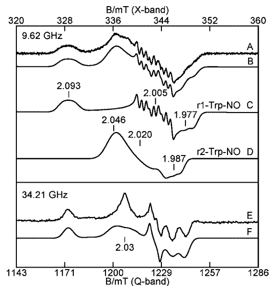
Figure 8. (A) X- and (E) Q-band EPR spectra of the NO adduct of 0.3 mM reduced TDO with 10 equiv of L-Trp. (B) Simulation sum (C) + (D) for the two sites, (C) simulation of r1-Trp-NO, (D) simulation of r2-Trp-NO, and (F) simulation sum for the two sites of (E). Experimental conditions: microwave frequencies as listed; power, 0.02 mW (X), 0.05 mW (Q); temperature, 20 K (X), 27 K (Q).
